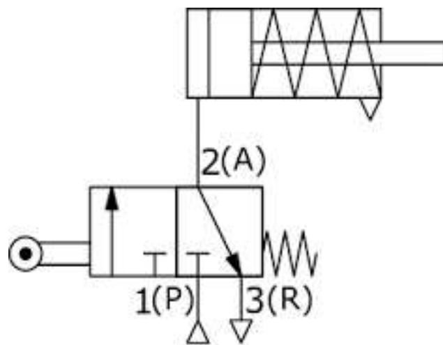
Single-acting cylinder drive
