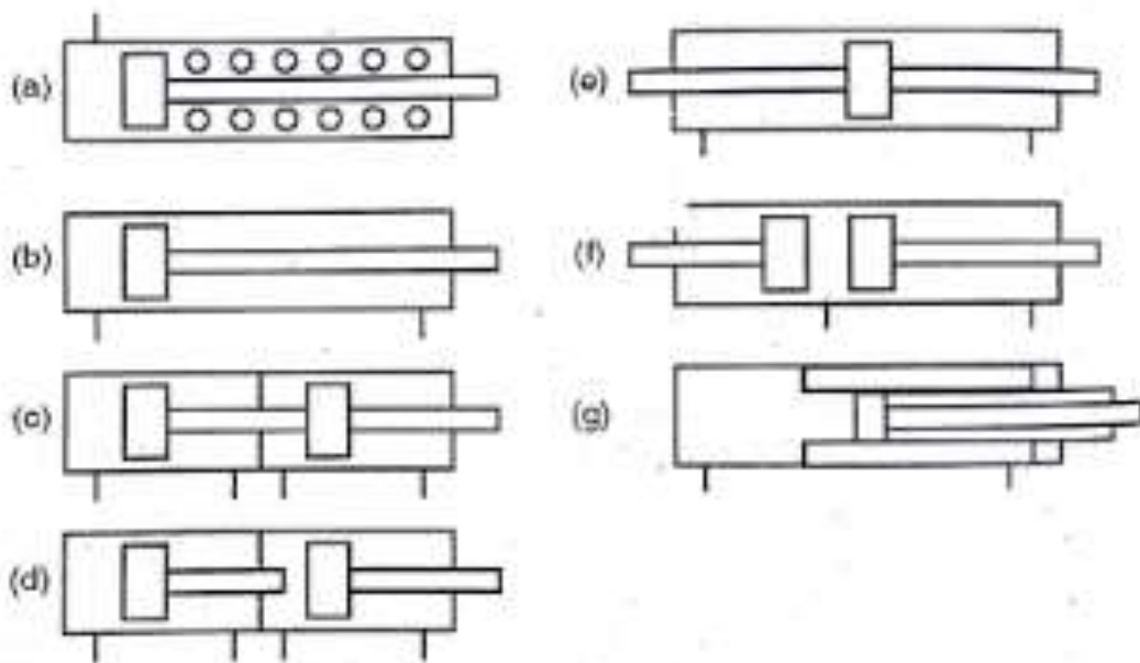
Figure 12.16 Basic Cylinder Types a) Single Acting Cylinder b) Double Acting Cylinder c) Tandem Cylinder d) Three Position Cylinder e) Through Rod Cylinder f) Adjustable Stroke Cylinder g) Telescoping Cylinder
