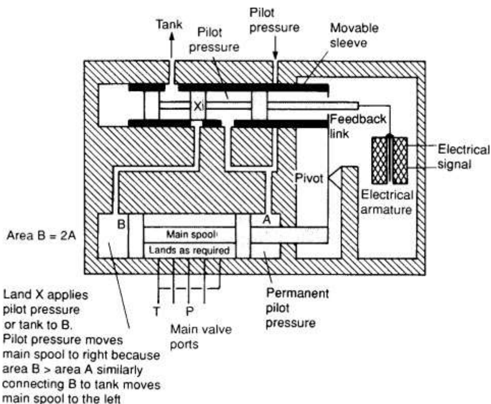
Simplified symbol for solenoid operated proportional valve with LVDT
