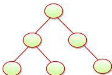
Fig. Complete-Binary Tree
