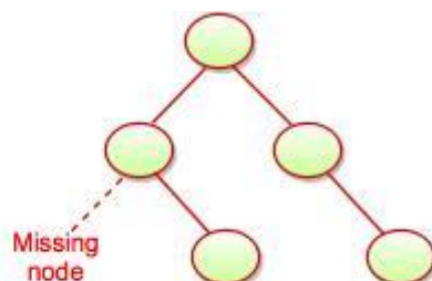
Fig. In-Complete-Binary Tree
