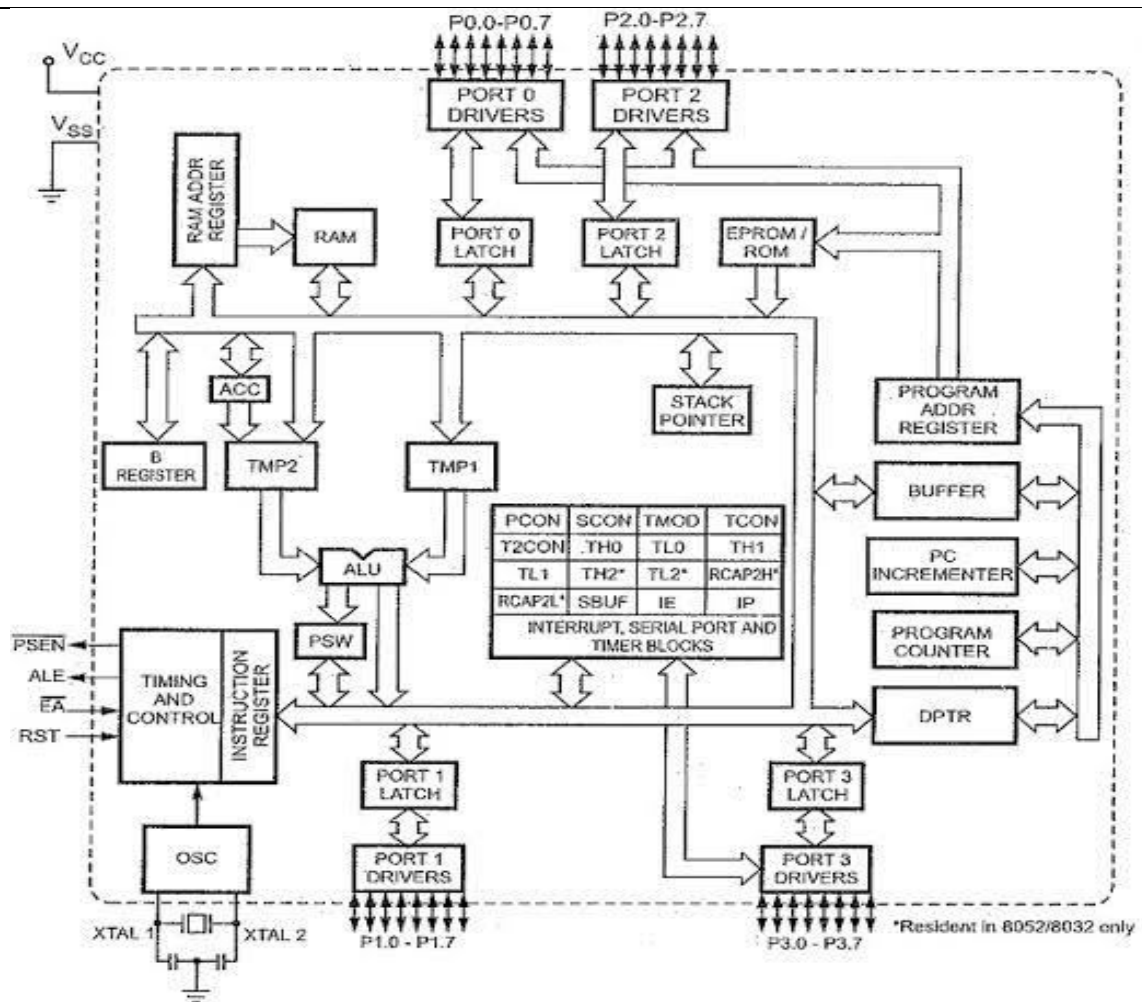
Fig. 12.2 Intel 8051/8031 architecture
